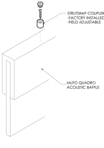
COUPLER
