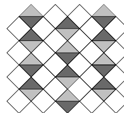
PATTERN 12 TRIANGLE 01 - QTY 12 TRIANGLE 01 - QTY 12 SQUARE 01 - QTY 24
